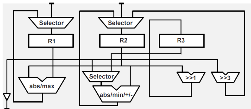
FIGURE 6.15 SRA design after register and unit merging
